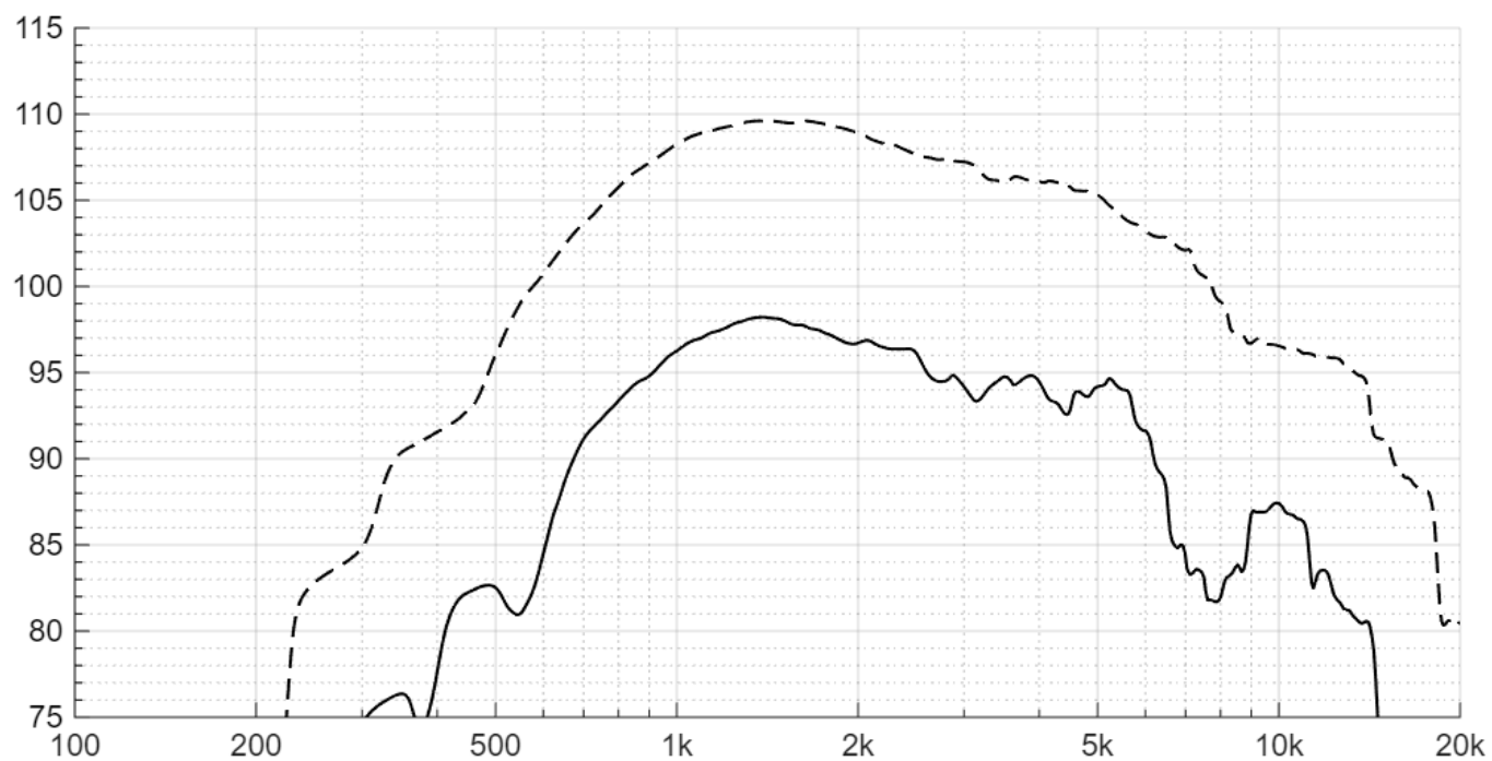
Fig. 2: Frequency response graph without EQ:
