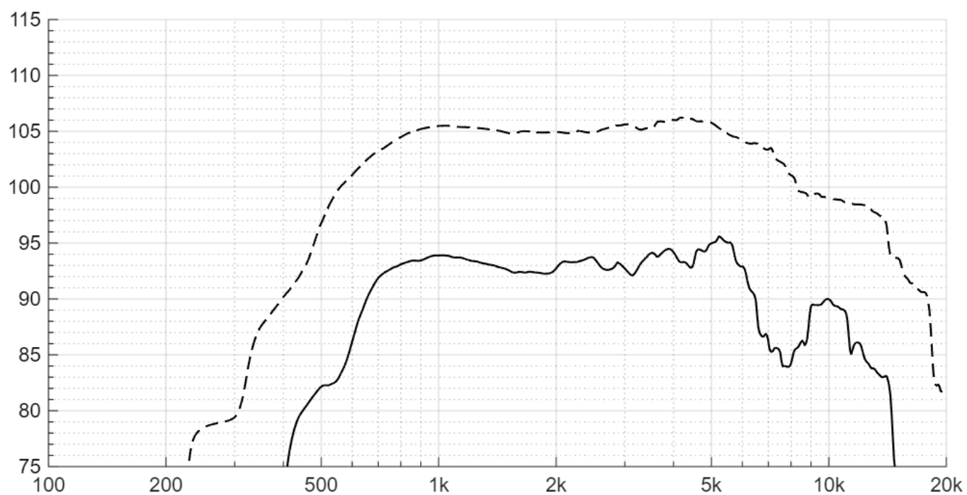
Fig. 3: Frequency response graph with EQ:
